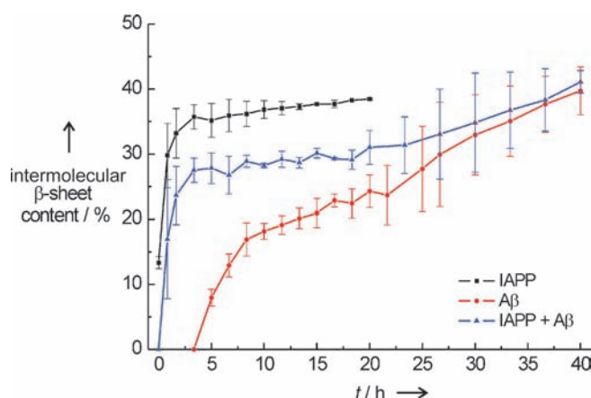
Figure 4. Time evolution of the intermolecular \beta -sheet content upon aggregation of 3 \mu\text{M} IAPP (black), 3 \mu\text{M} A \beta (red) and an equimolar IAPP-A \beta mixture (3 \mu\text{M} each, blue) at T=25^\circ\text{C} in the presence of an anionic lipid raft bilayer, derived from peak fitting of the normalized ATR-FTIR spectra.
